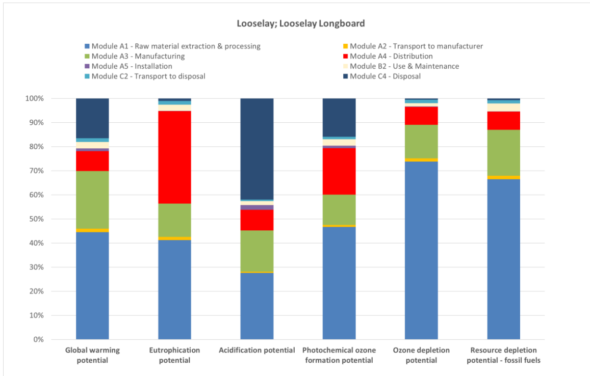
Figure 2. Contribution analysis for the Karndean Designflooring LVT flooring products (excluding product replacements) over the product's RSL – CML-IA, Product distribution to the United Kingdom.
