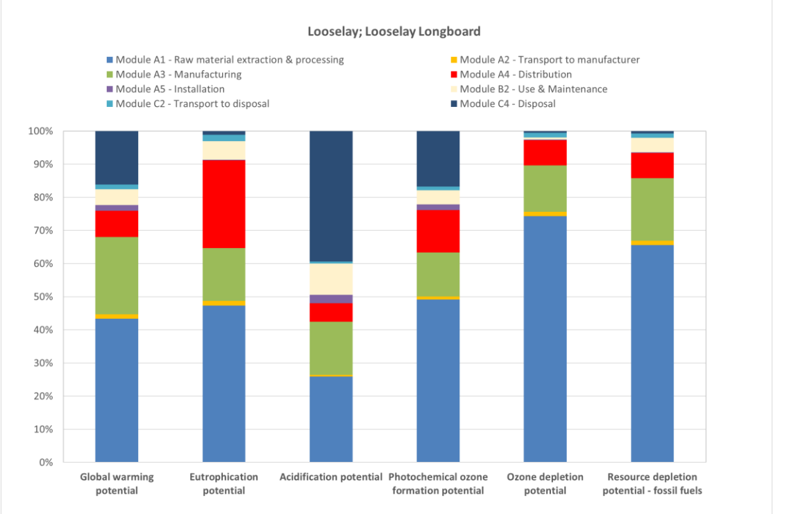
Figure 4. Contribution analysis for the Karndean Designflooring LVT flooring products (excluding product replacements) over the product's RSL – CML-IA. Product distribution to Australia.
