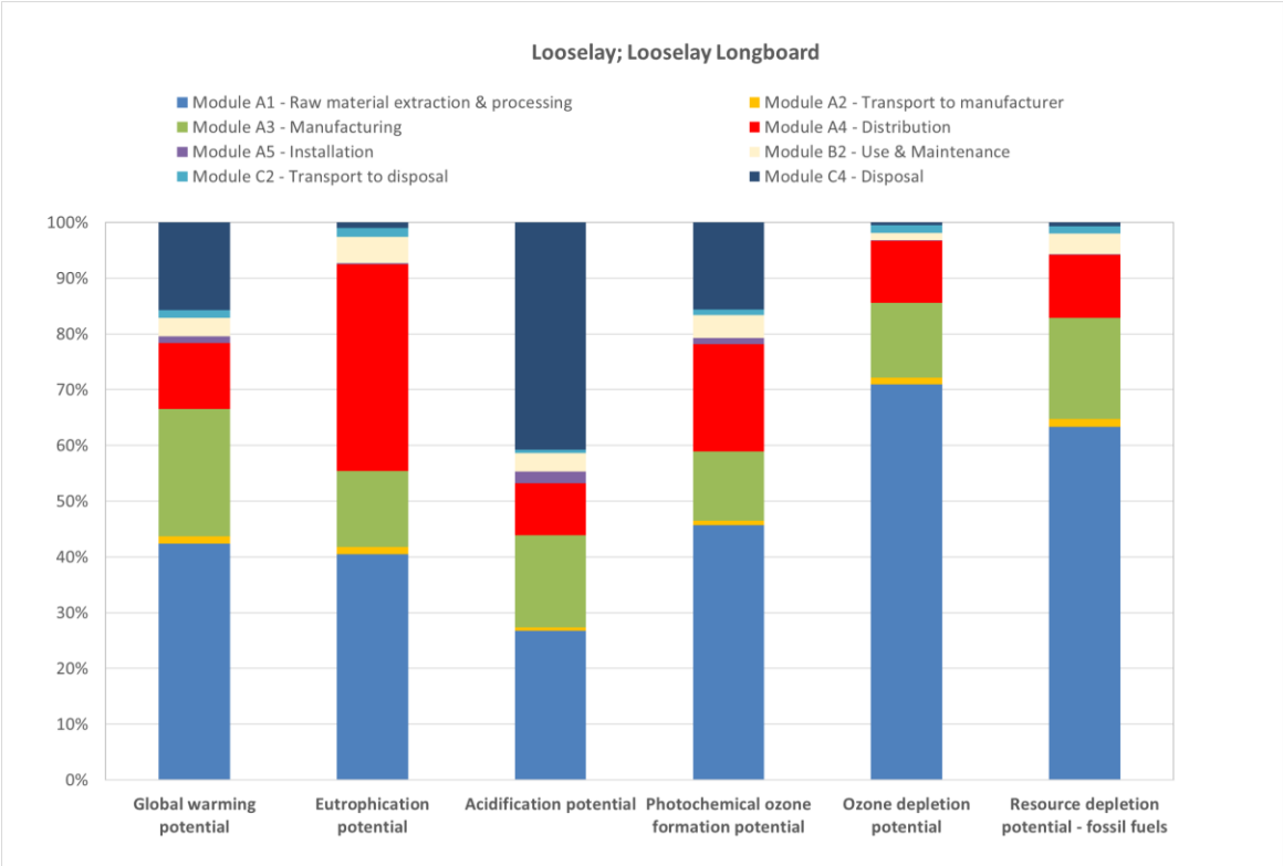
Figure 3. Contribution analysis for the Karndean Designflooring LVT flooring products (excluding product replacements) over the product's RSL – CML-IA. Product distribution to North America.
