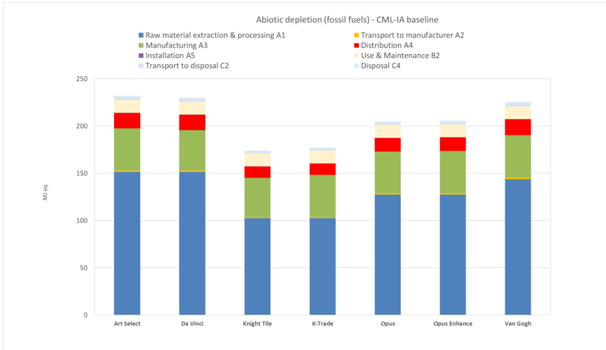
Figure 19. Contribution analysis for the Karndean Designflooring luxury vinyl flooring products (excluding product replacements) over the product's RSL – Abiotic Depletion Potential (fossil fuels) – CML-IA. Product distribution to Australia.
