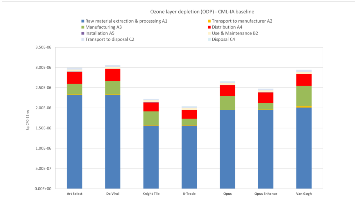
Figure 11. Contribution analysis for the Karndean Designflooring luxury vinyl flooring products (excluding product replacements) over the product's RSL – Ozone Layer Depletion Potential – CML-IA. Product distribution to North America.
