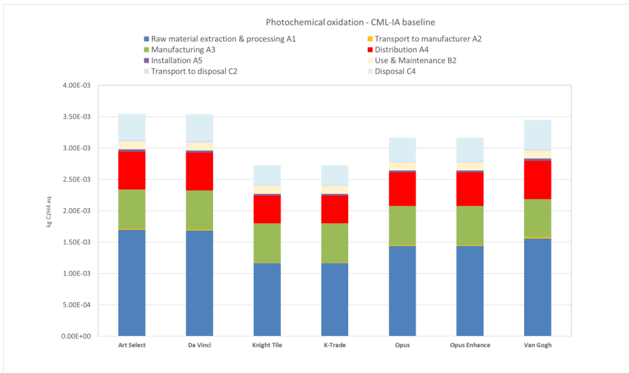
Figure 6. Contribution analysis for the Karndean Designflooring luxury vinyl flooring products (excluding product replacements) over the product's RSL – Photochemical Oxidation Potential – CML-IA. Product distribution to the United Kingdom.
