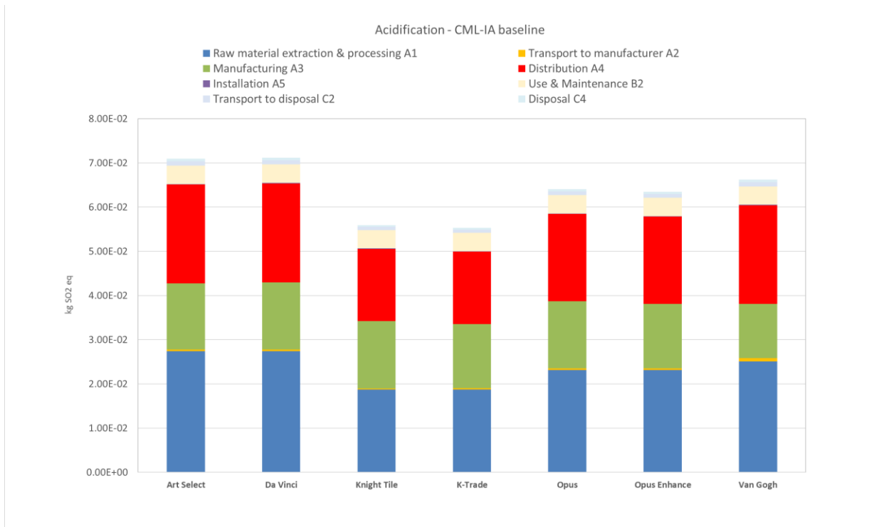
Figure 9. Contribution analysis for the Karndean Designflooring luxury vinyl flooring products (excluding product replacements) over the product's RSL – Acidification Potential – CML-IA. Product distribution to North America.
