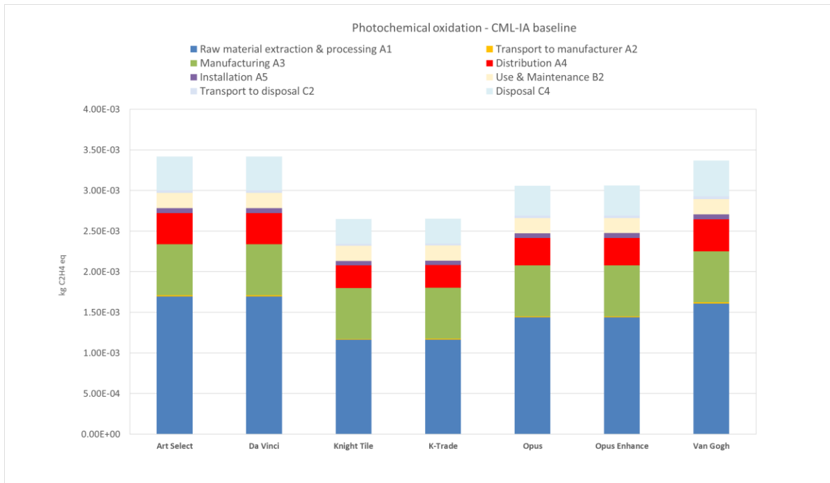
Figure 18. Contribution analysis for the Karndean Designflooring luxury vinyl flooring products (excluding product replacements) over the product's RSL – Photochemical Oxidation Potential – CML-IA. Product distribution to Australia.
