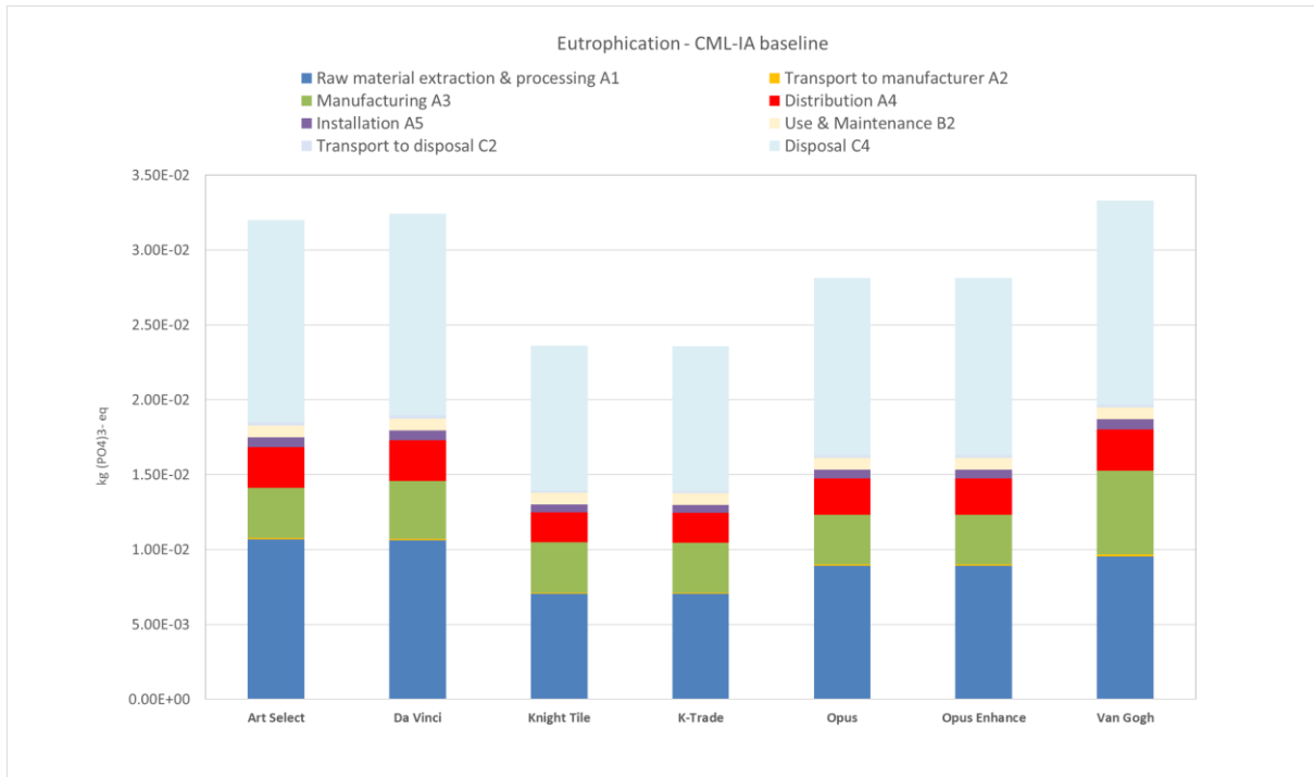
Figure 4. Contribution analysis for the Karndean Designflooring luxury vinyl flooring products (excluding product replacements) over the product's RSL – Eutrophication Potential – CML-IA. Product distribution to the United Kingdom.
