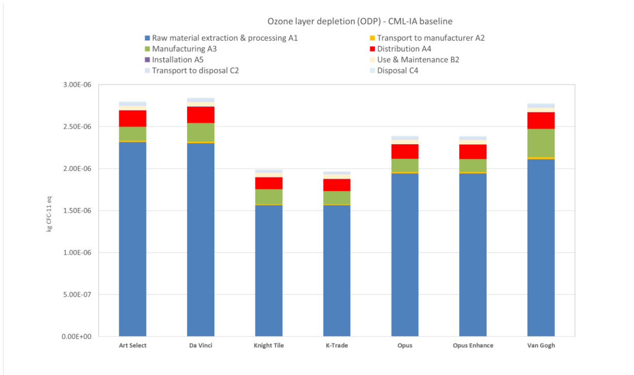
Figure 5. Contribution analysis for the Karndean Designflooring luxury vinyl flooring products (excluding product replacements) over the product's RSL – Ozone Layer Depletion Potential – CML-IA. Product distribution to the United Kingdom.
