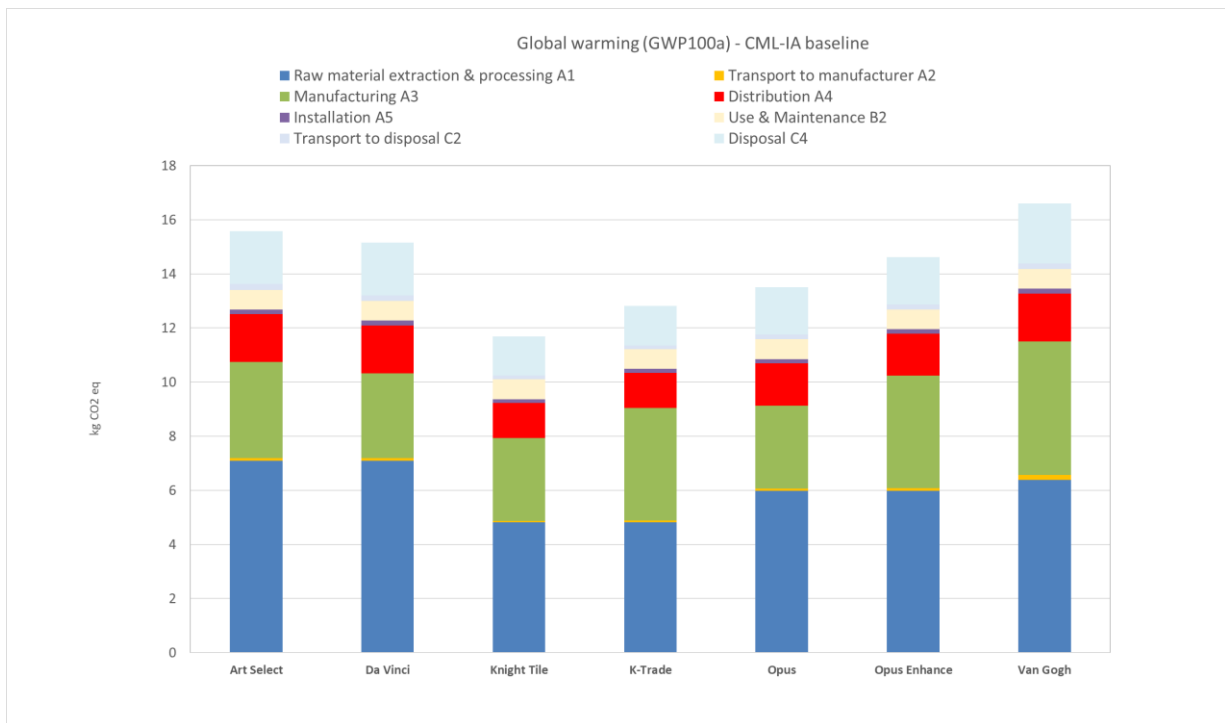
Figure 8. Contribution analysis for the Karndean Designflooring luxury vinyl flooring products (excluding product replacements) over the product's RSL – Global Warming Potential – CML-IA. Product distribution to North America.
