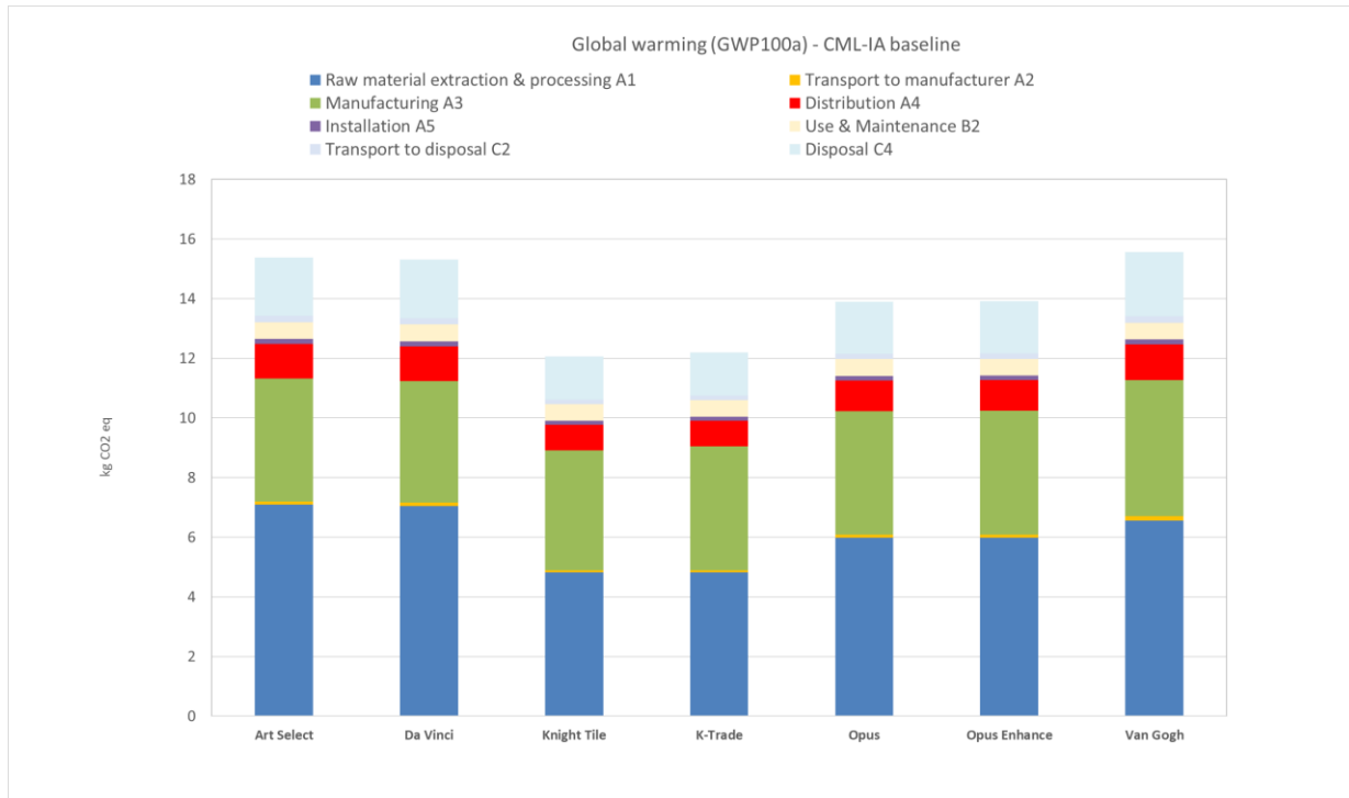
Figure 2. Contribution analysis for the Karndean Designflooring luxury vinyl flooring products (excluding product replacements) over the product's RSL – Global Warming Potential – CML-IA. Product distribution to the United Kingdom.
