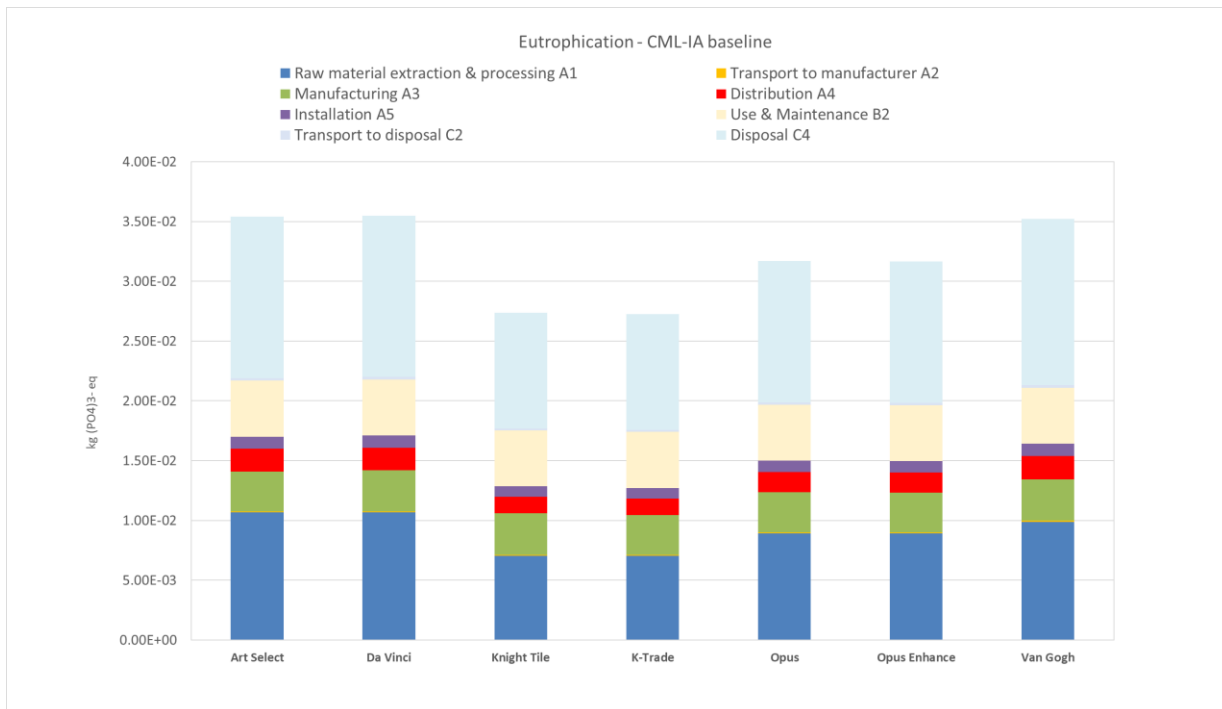
Figure 16. Contribution analysis for the Karndean Designflooring luxury vinyl flooring products (excluding product replacements) over the product's RSL – Eutrophication Potential – CML-IA. Product distribution to Australia.
