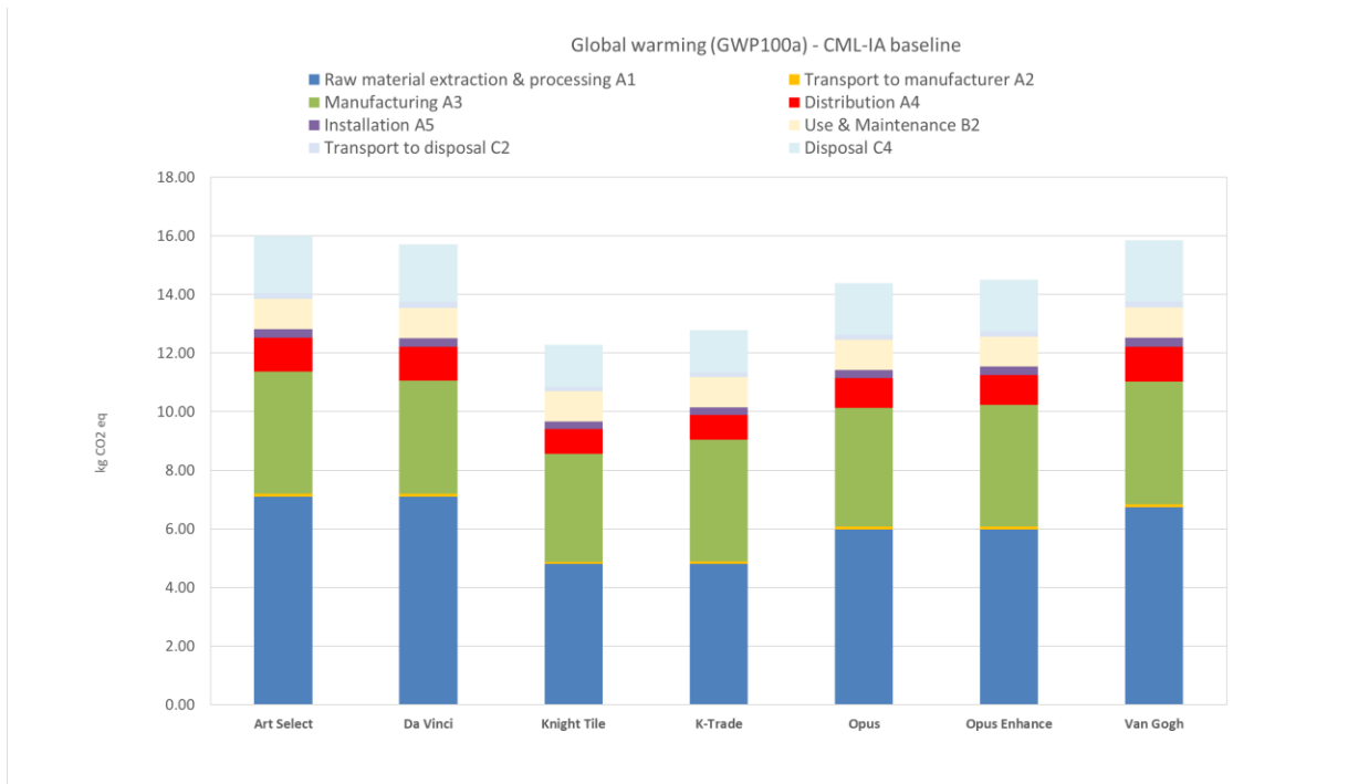
Figure 14. Contribution analysis for the Karndean Designflooring luxury vinyl flooring products (excluding product replacements) over the product's RSL – Global Warming Potential – CML-IA. Product distribution to Australia.
