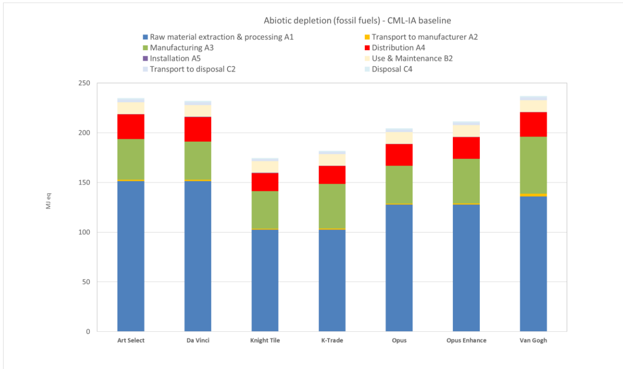
Figure 13. Contribution analysis for the Karndean Designflooring luxury vinyl flooring products (excluding product replacements) over the product's RSL – Abiotic Depletion Potential (fossil fuels) – CML-IA. Product distribution to North America.
