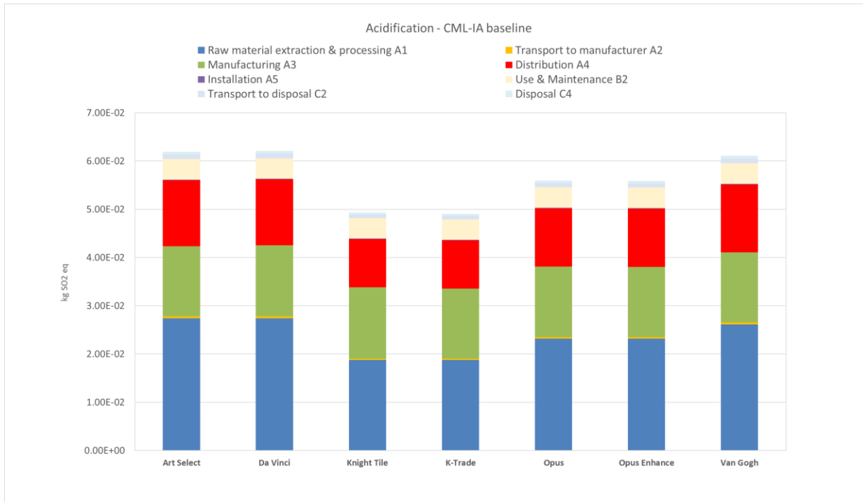
Figure 15. Contribution analysis for the Karndean Designflooring luxury vinyl flooring products (excluding product replacements) over the product's RSL – Acidification Potential – CML-IA. Product distribution to Australia.
