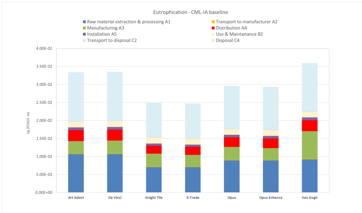
Figure 10. Contribution analysis for the Karndean Designflooring luxury vinyl flooring products (excluding product replacements) over the product's RSL – Eutrophication Potential – CML-IA. Product distribution to North America.
