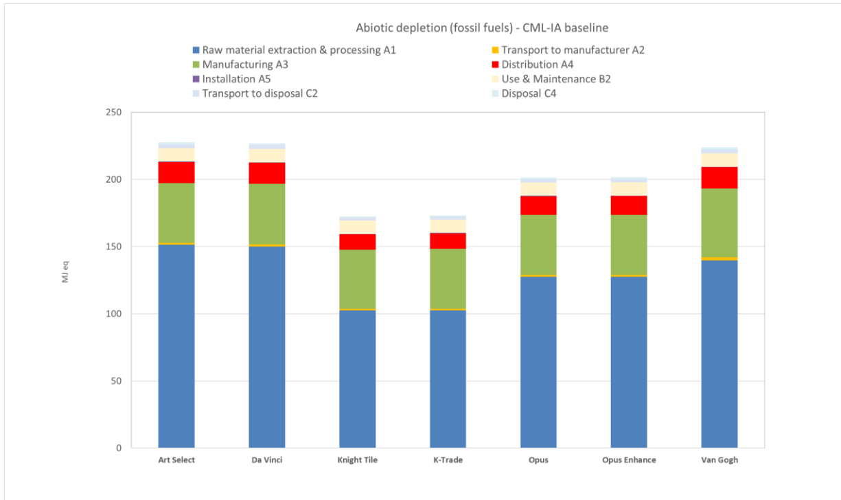
Figure 7. Contribution analysis for the Karndean Designflooring luxury vinyl flooring products (excluding product replacements) over the product's RSL – Abiotic Depletion Potential (fossil fuels) – CML-IA. Product distribution to the United Kingdom.
